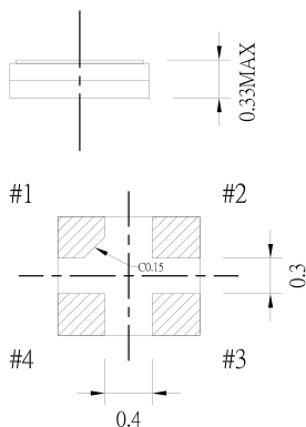
Example of a Terminal Land Pattern
